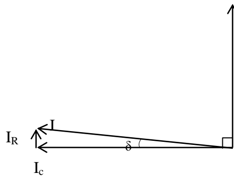
Figure 2 :Tan Delta
