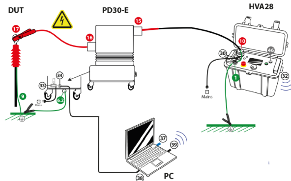
Figure 7: PD Measurement setup
