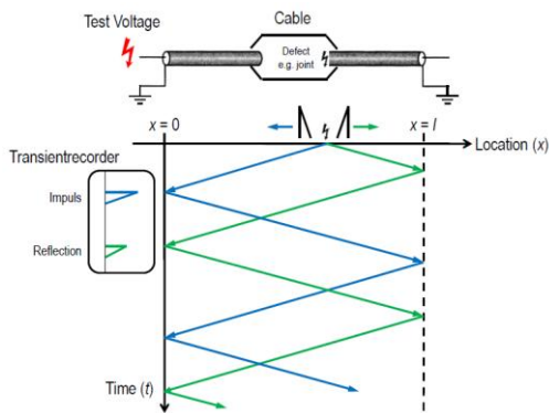
Figure 5: PD pulse travel diagram
