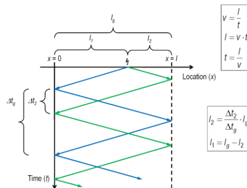
Figure 6: Distance to PD calculation
