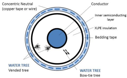
Figure 3: Typical XLPE cable
